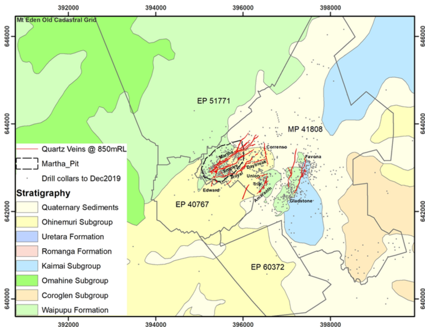
Figure 4: Drill Hole Location Plan
