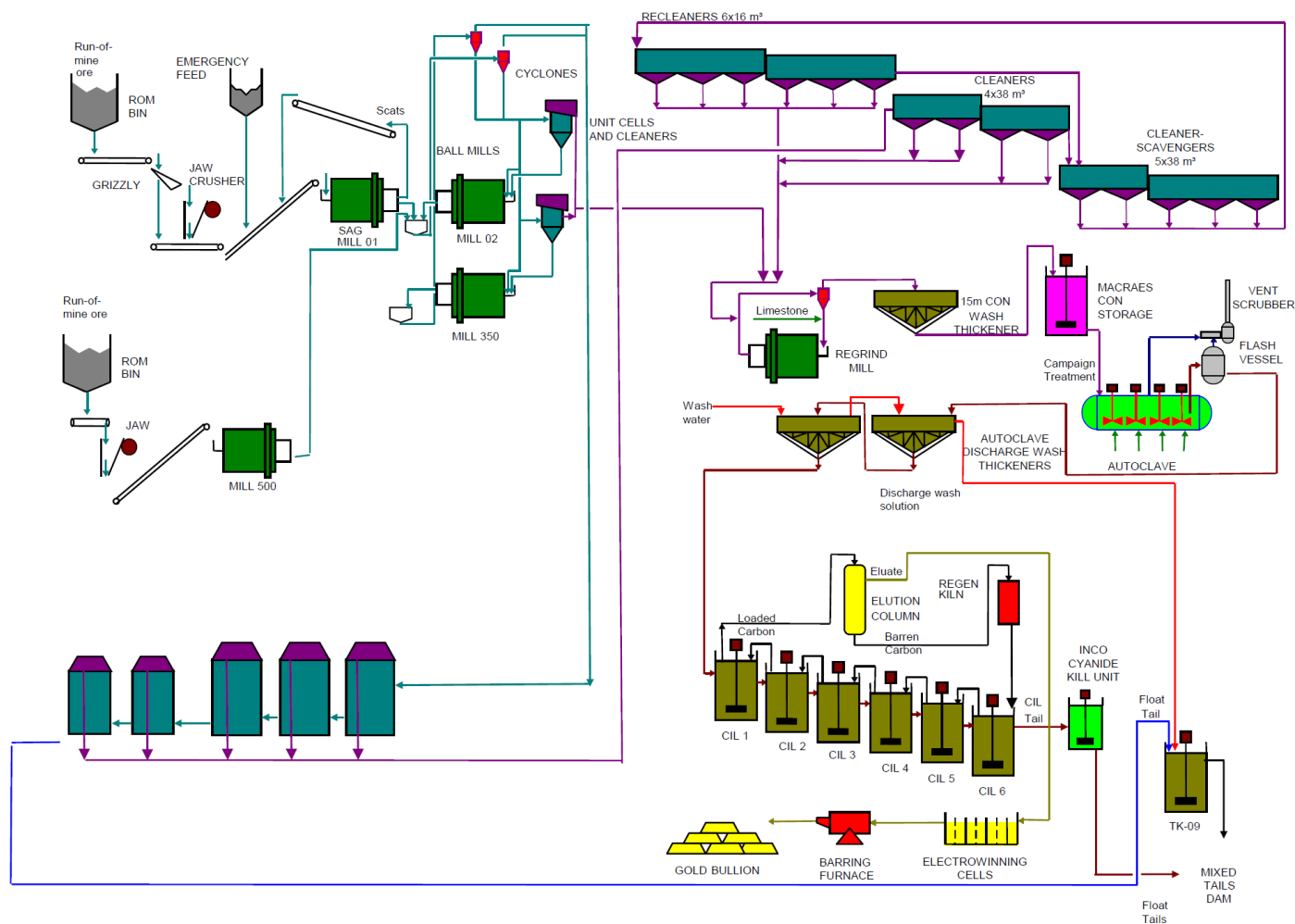
MACRAES PROCESSING PLANT FLOWSHEET
