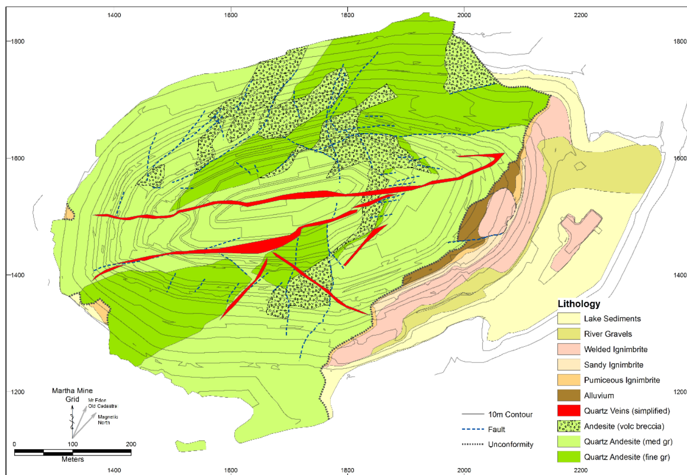
Figure 2: Geological Plan, Martha Area
