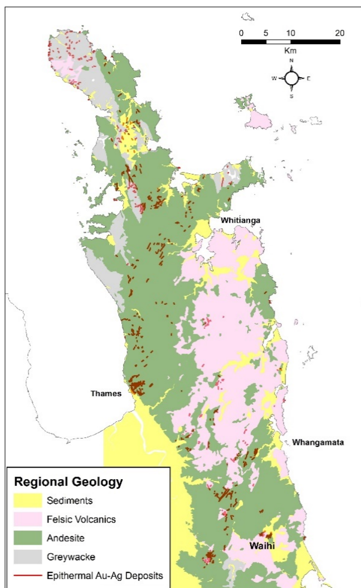
Figure 1: Regional Geological Plan
